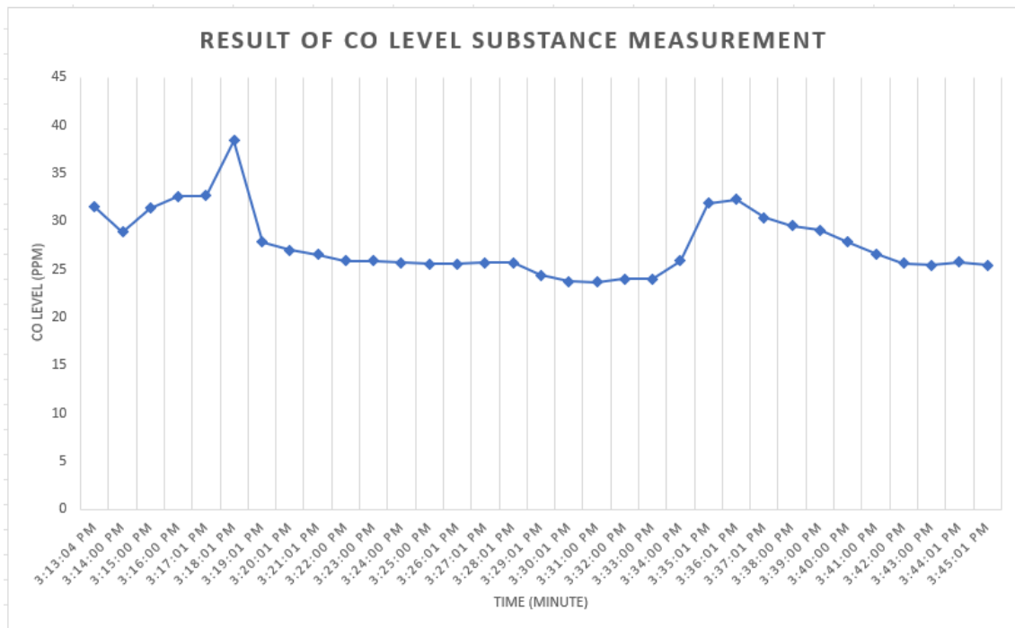
Figure 4. Graph of CO substance level measurement in the room
