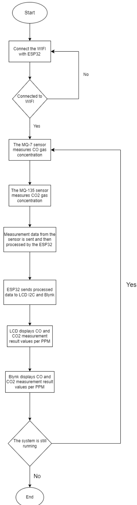
Figure 2. Flowchart of the system
